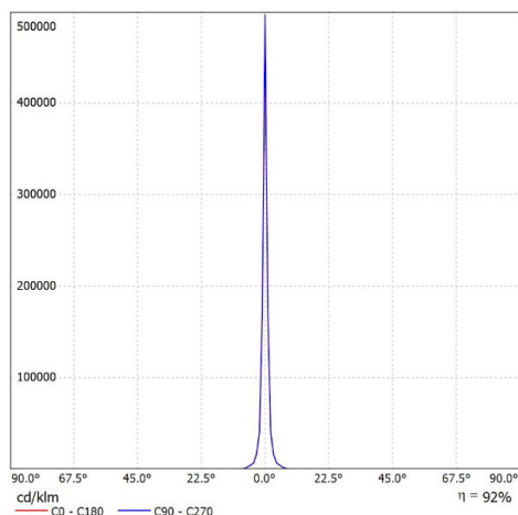
Luminaire: Ledil Oy FCP13895_SEANNA-A_(XHP35_HI)_SIMULATED Lamps: 1 x Cree XHP35 HI
